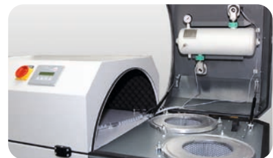
The top of the filter module is hinged so as to provide convenient access for service and maintenance work.
